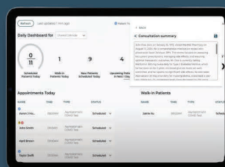
Pharmacist Forms
