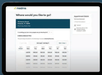
Appointment Scheduler
